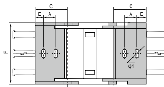
X 1 型接头 X 1 type bracket
