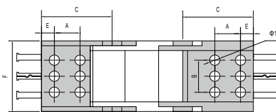
X 8 型接头 X 8 type bracket
